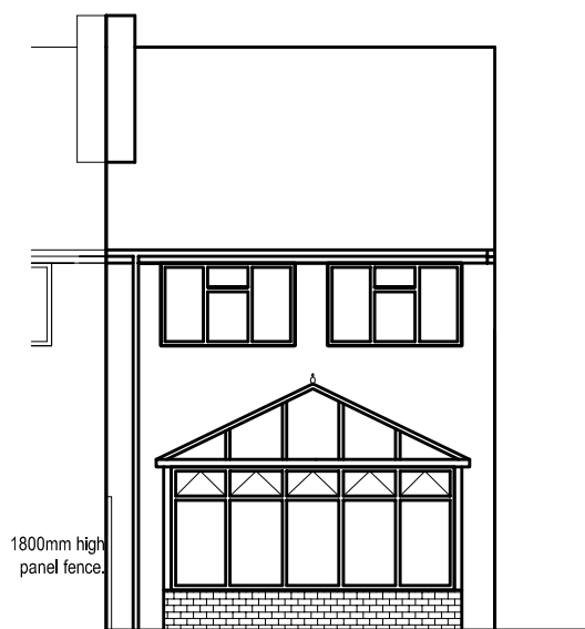
REAR ELEVATION AS PROPOSED (1:100)
