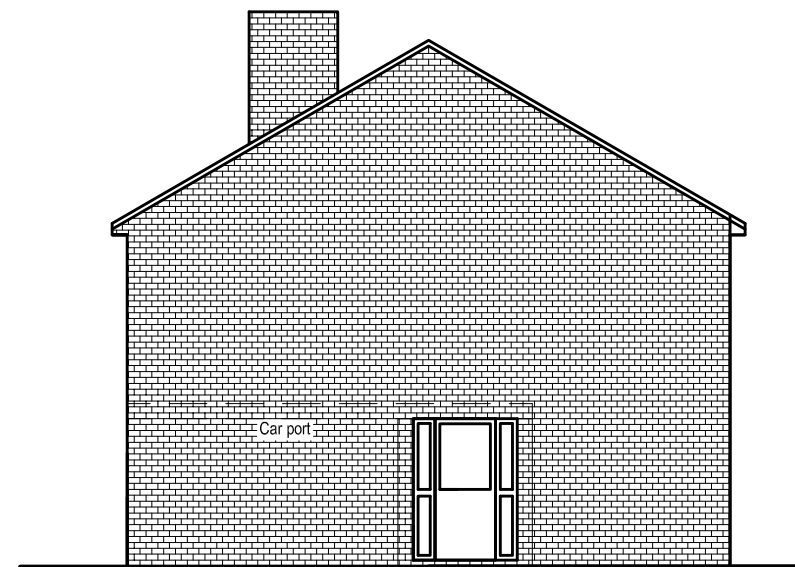
SIDE ELEVATION AS EXISTING (1:100)
