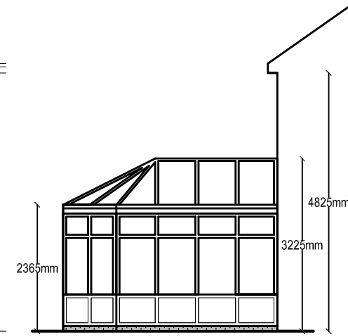
SIDE ELEVATION AS PROPOSED (1:100)
