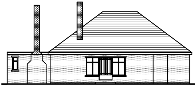
SIDE ELEVATION AS EXISTING (1:100)
