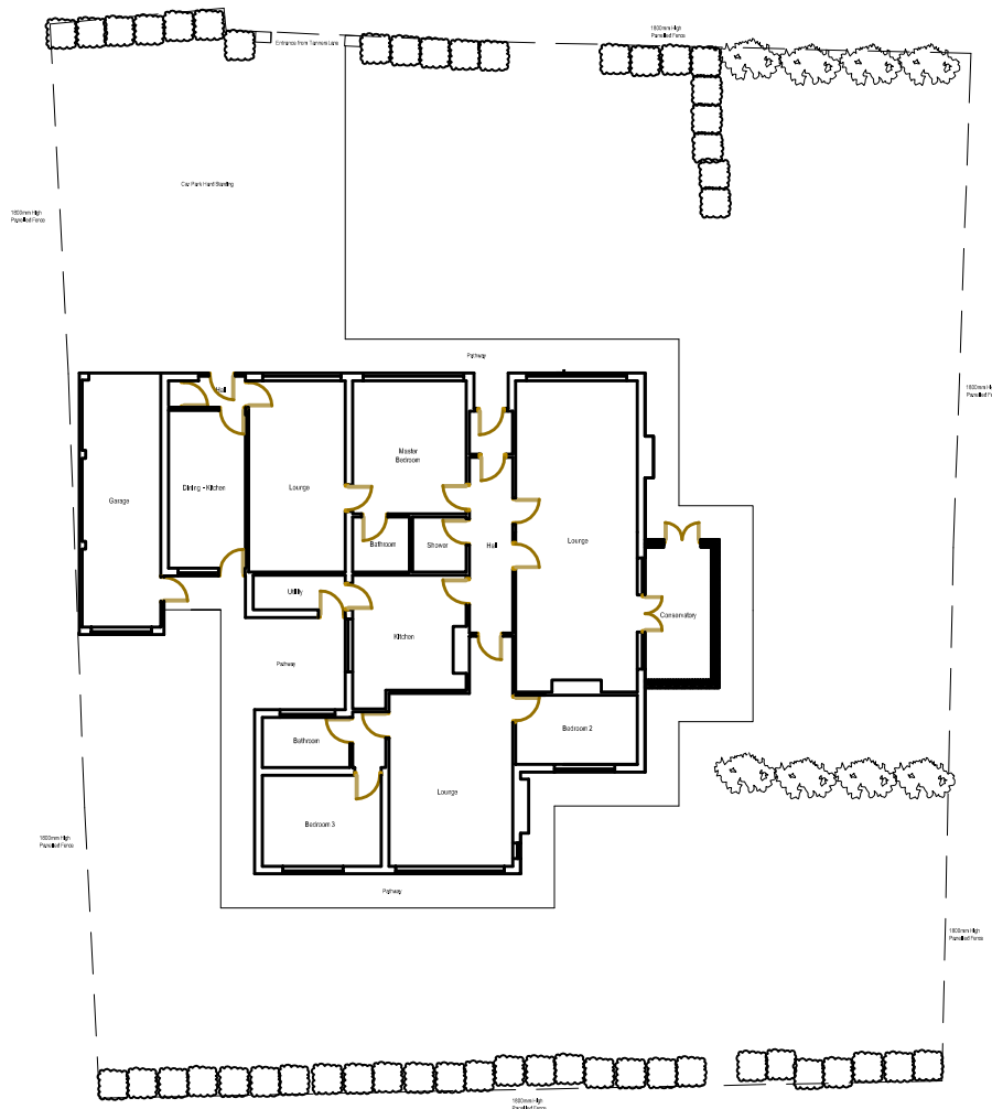
GROUND FLOOR PLAN AS PROPOSED (1:200)
