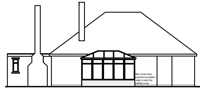
SIDE ELEVATION AS PROPOSED (1:100)
